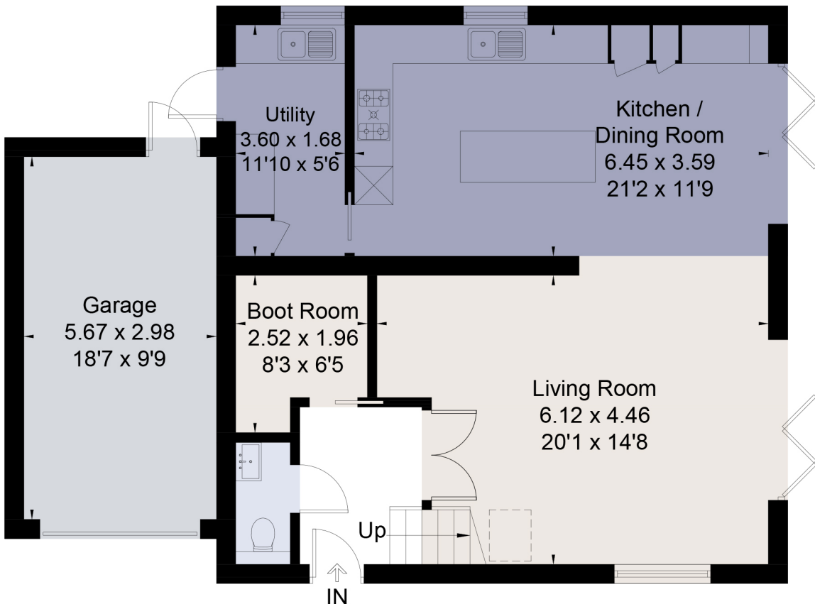
Ground Floor
