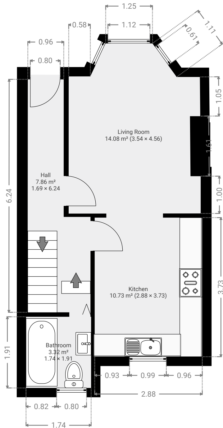
Raised Ground Floor
