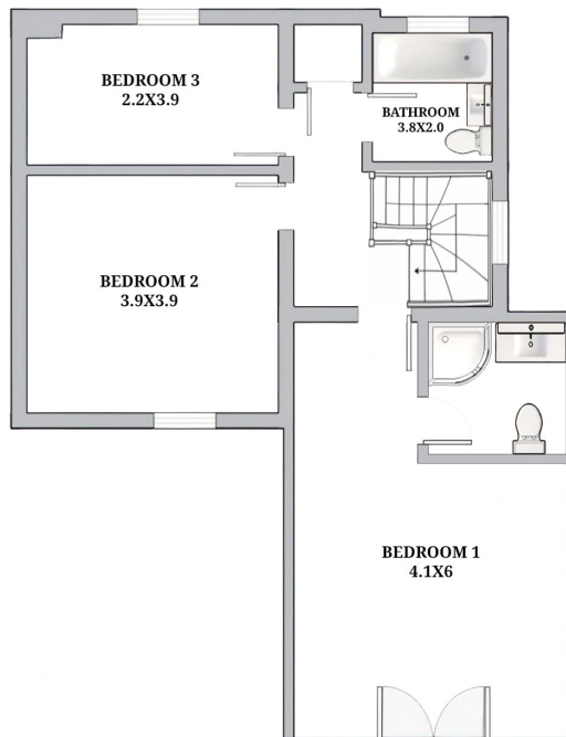
1ST FLOOR PLAN TOTAL AREA : 136 SQM
